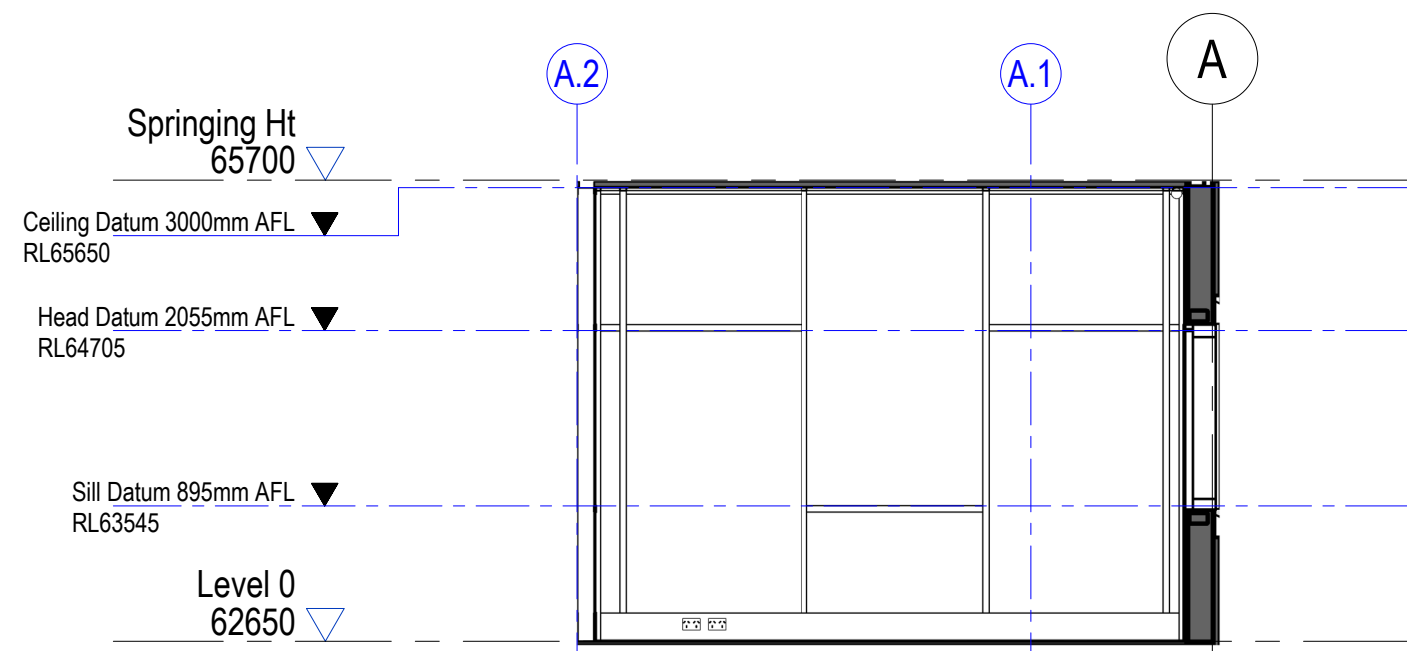
4 0.18 - First Aid - South Elevation 1 : 50
