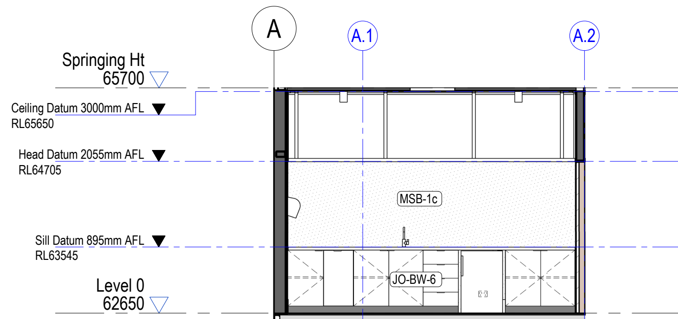
2 0.18 - First Aid - North Elevation 1 : 50
