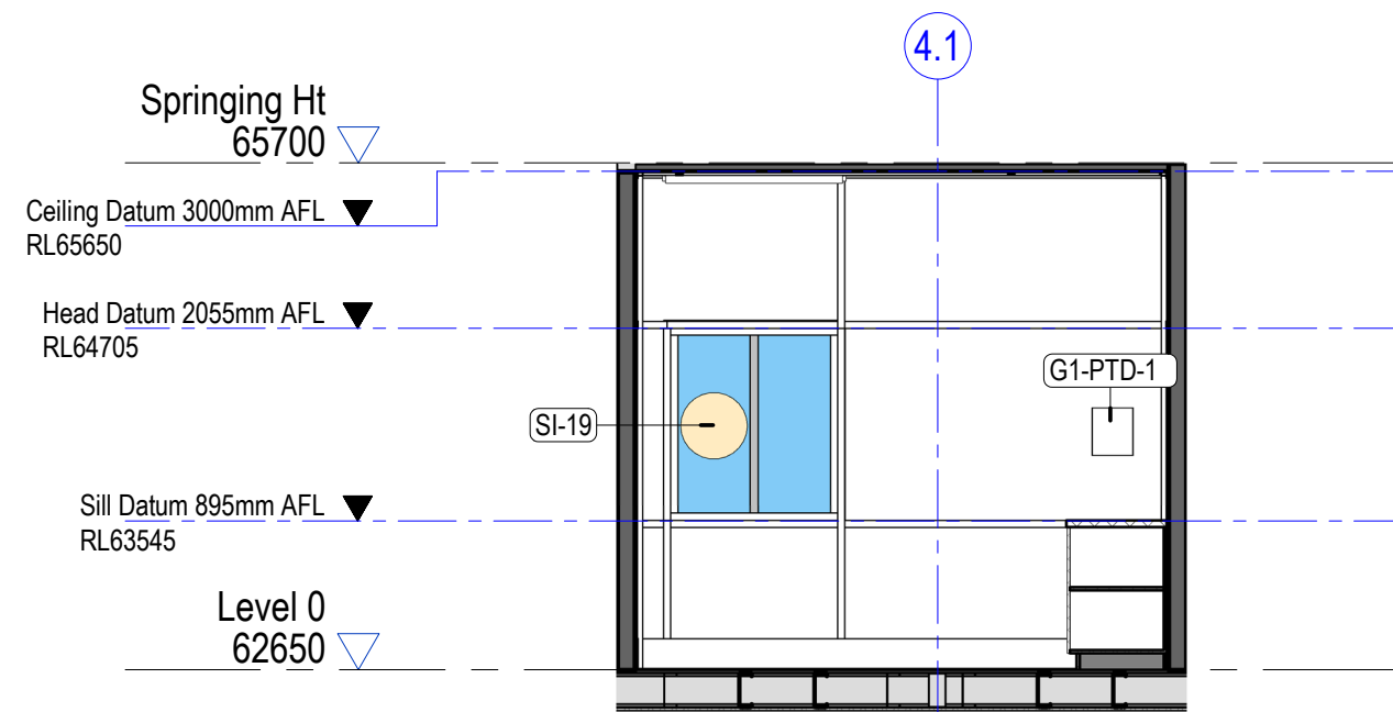
5 0.18 - First Aid - West Elevation 1 : 50
