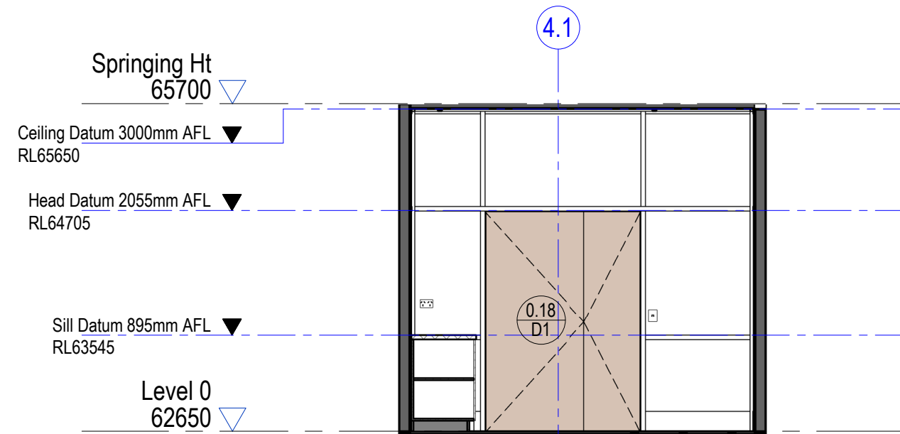
3 0.18 - First Aid - East Elevation 1 : 50
